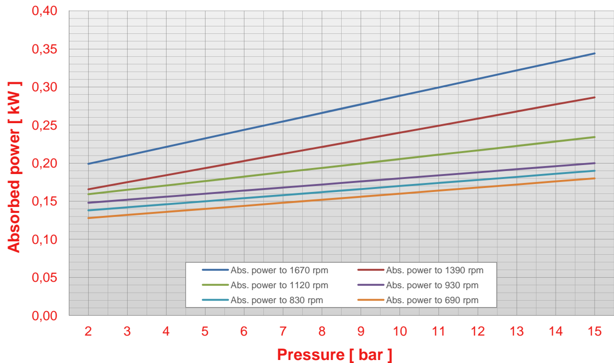
Pump S 05 pressure - abs. power chart (viscosity 50 cps)
