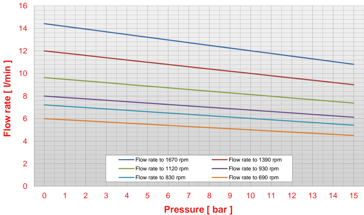
Pump SK 10 pressure - flow rate chart (viscosity 50 cps)
