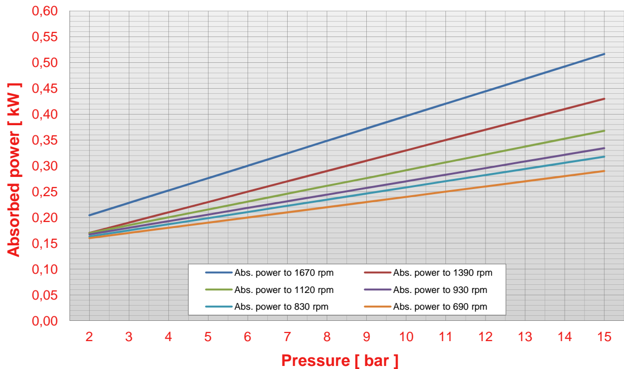
Pump SK 10 pressure - abs. power chart (viscosity 50 cps)
