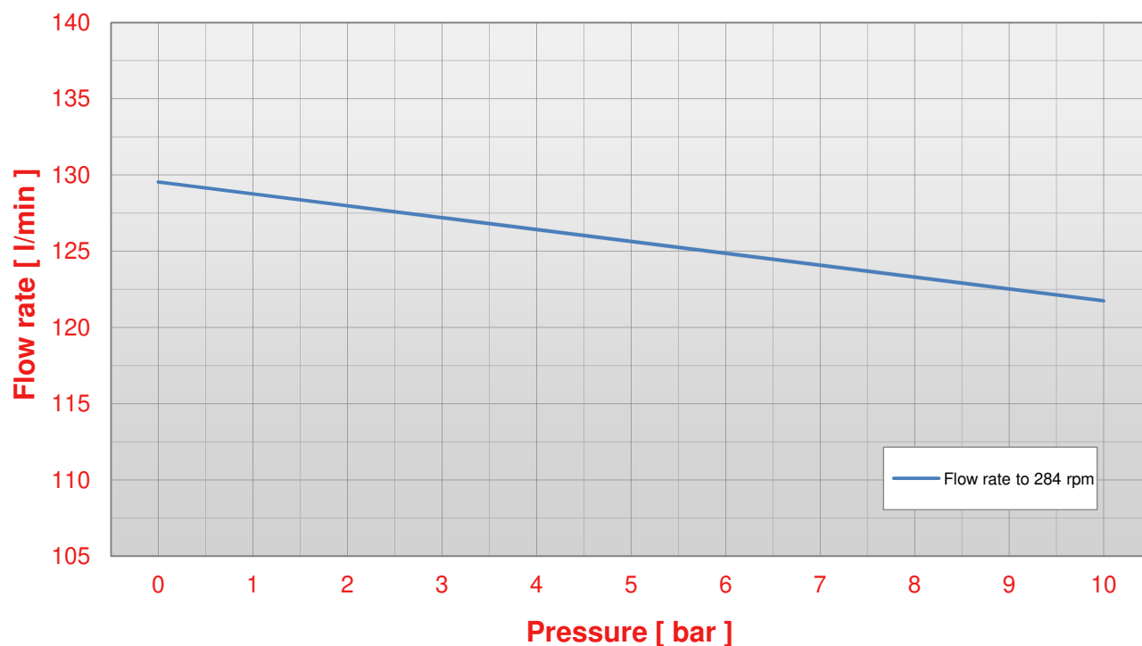
Pump S 800 pressure - flow rate chart (viscosity 600 cps)
