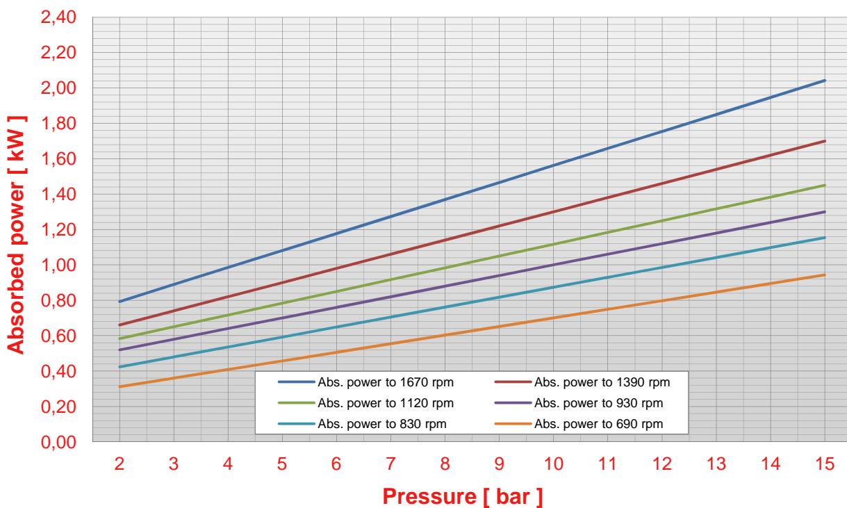
Pump S 50 pressure - abs. power chart (viscosity 50 cps)
