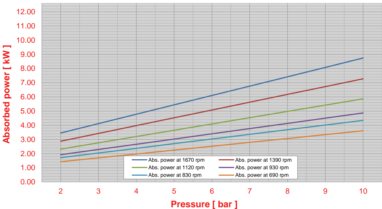
Pump S 300 pressure - abs. power chart (viscosity 50 cps)
