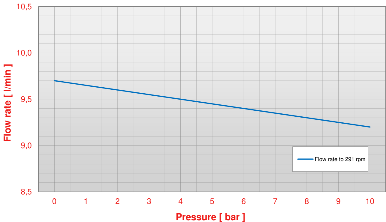
Pump S 50 pressure - flow rate chart (viscosity 600 cps)
