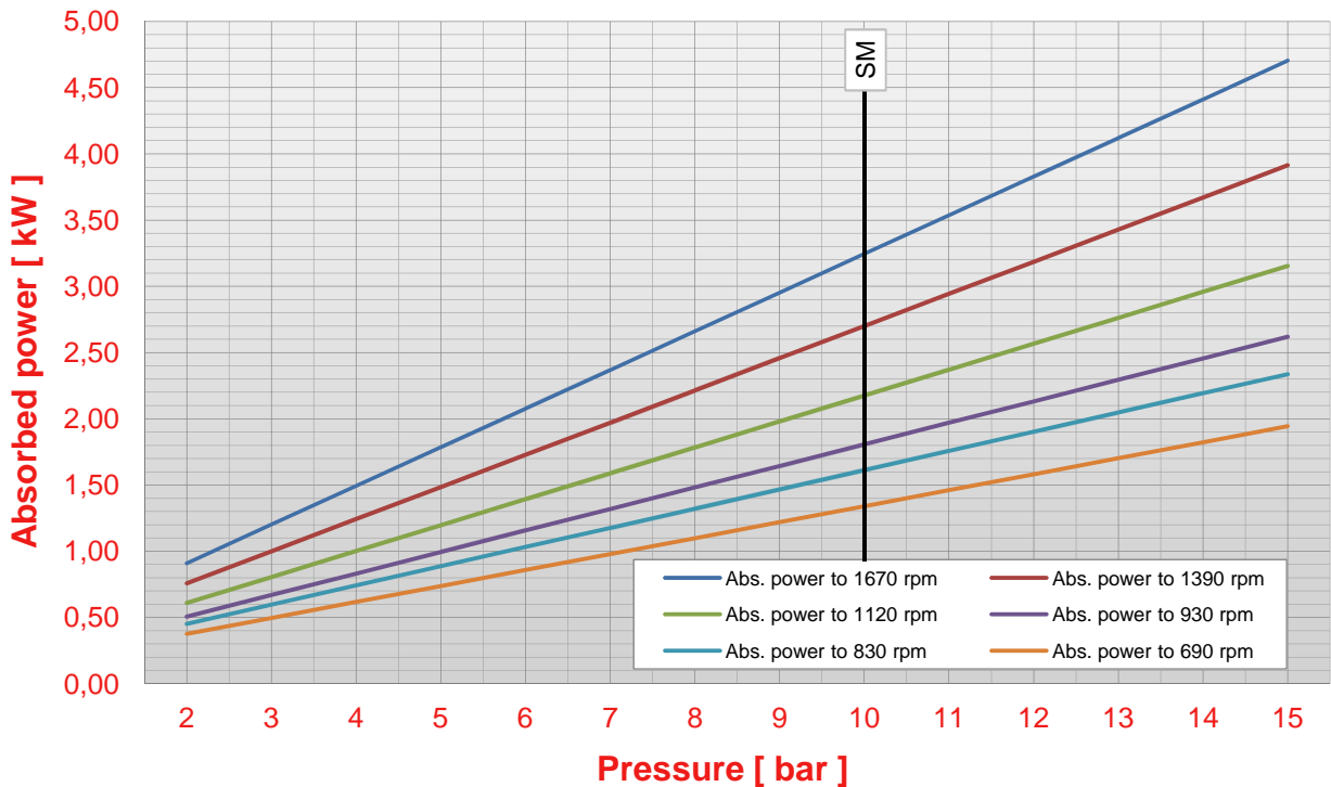
Pump S 100 pressure - abs. power chart (viscosity 50 cps)
