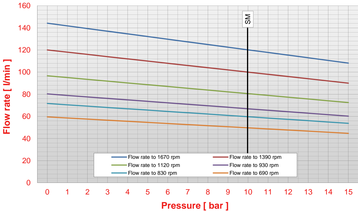
Pump S 100 pressure - flow rate chart (viscosity 50 cps)
