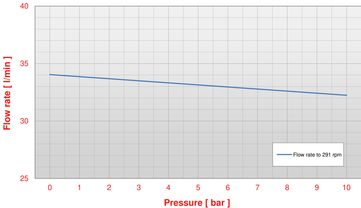
Pump S 150 pressure - flow rate chart (viscosity 600 cps)
