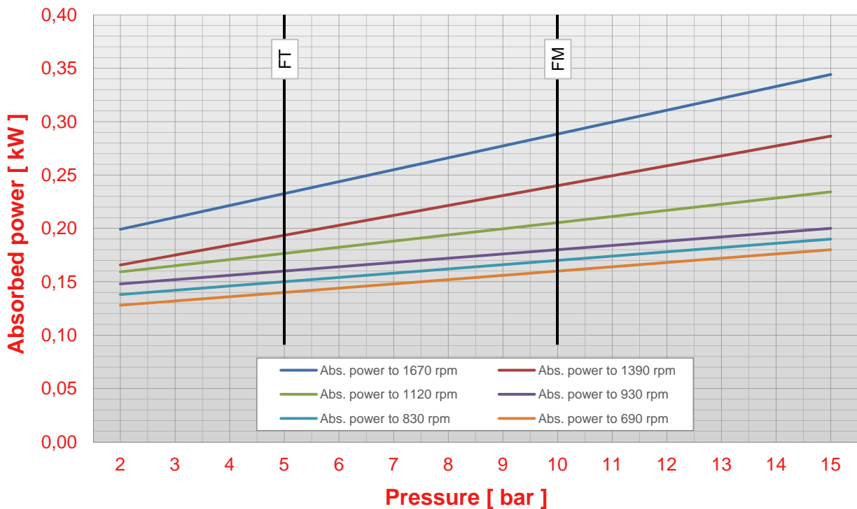
Pump F FT FM 05 pressure - abs. power chart (viscosity 50 cps)
